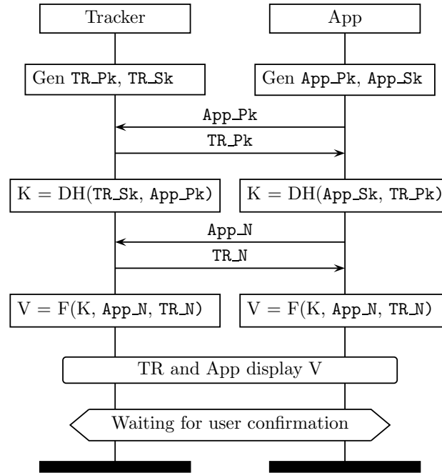
Figure 9: Authenticated key establishment (i.e., pairing) protocol providing C1+C2. Tracker and app generate a public-private key pair and share the public keys ( App_Pk and TR_Pk ) with each other. They calculate a new key through a Diffie–Hellman (DH) function and share two nonces ( App_N and TR_N ). Then, the tracker and the app both calculate a confirmation value ( V ) displayed on each screen and wait for user confirmation concerning the match of the displayed values. The DH function guarantees C1, while the user verifying tracker and app during pairing confirmation guarantees C2.
